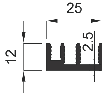
1263 0.412 Kg / m
