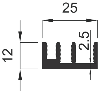
1262 0.377 Kg / m
