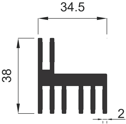
1021 1.260 Kg / m
