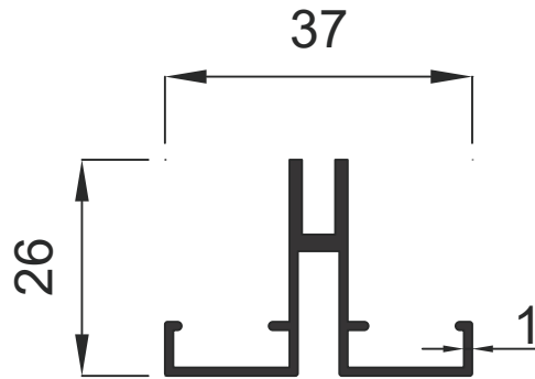
1952 0.320 Kg / m
