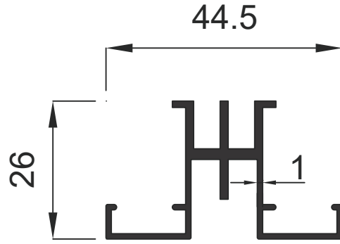
1953 0.445 Kg / m
