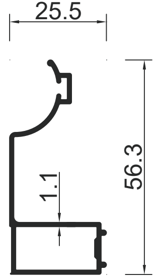
1776 0.410 Kg / m
