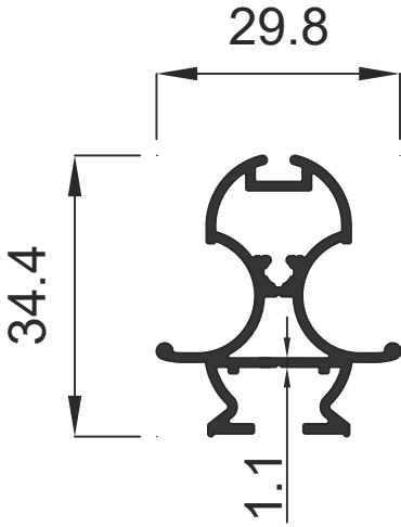
1768 0.461 Kg / m
