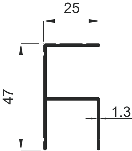
1781 0.401 Kg / m
