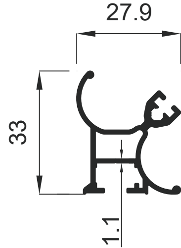
1772 0.423 Kg / m
