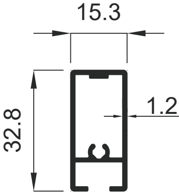
1778 0.352 Kg / m
