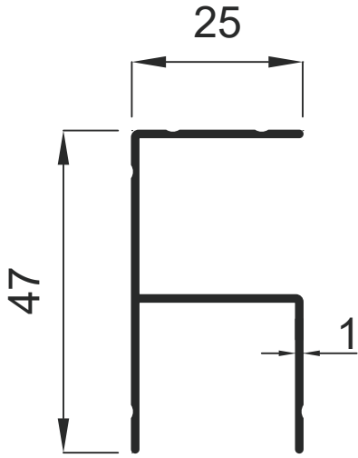
936 0.312 Kg / m
