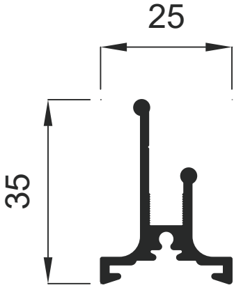
1599 0.396 Kg / m
