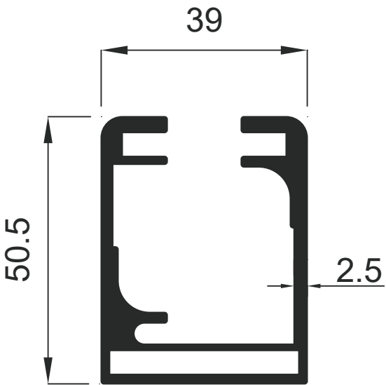
1593 1.385 Kg / m
