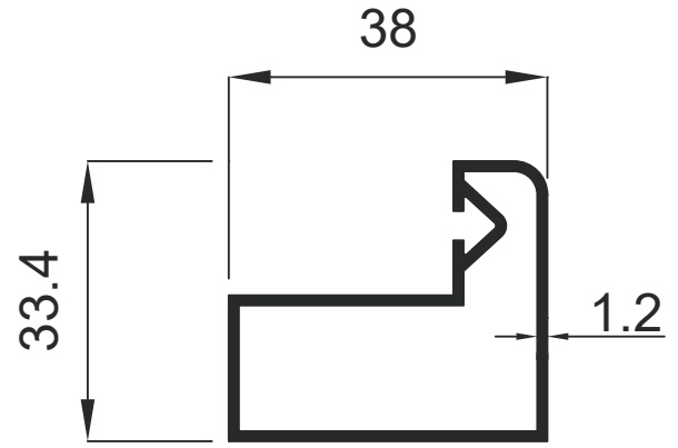
1838 0.474 Kg / m
