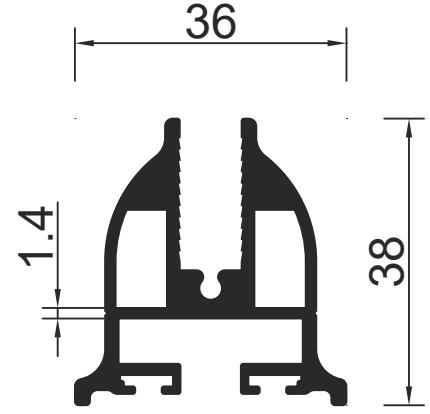
1595 0.970 Kg / m
