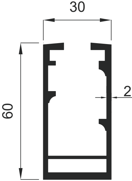
1573 1.176 Kg / m
