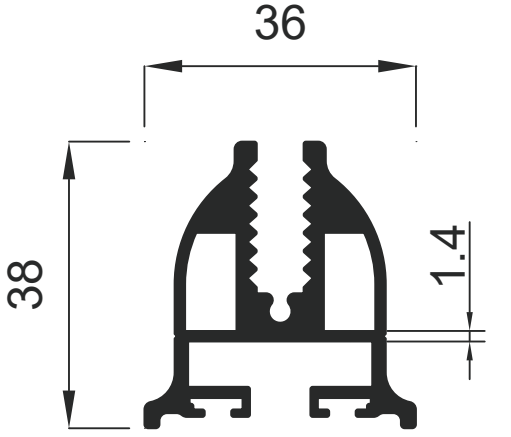
1592 1.040 Kg / m
