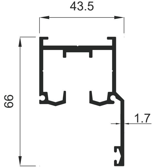
1597 0.981 Kg / m
