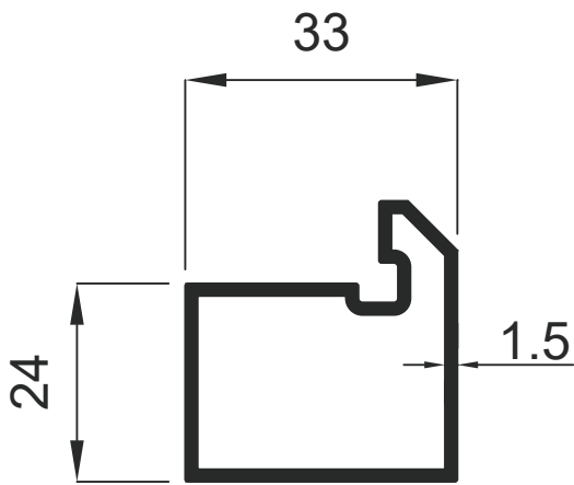
1701 0.537 Kg / m
