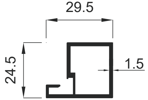
1574 0.401 Kg / m
