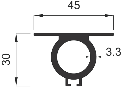
1392 0.839 Kg / m
